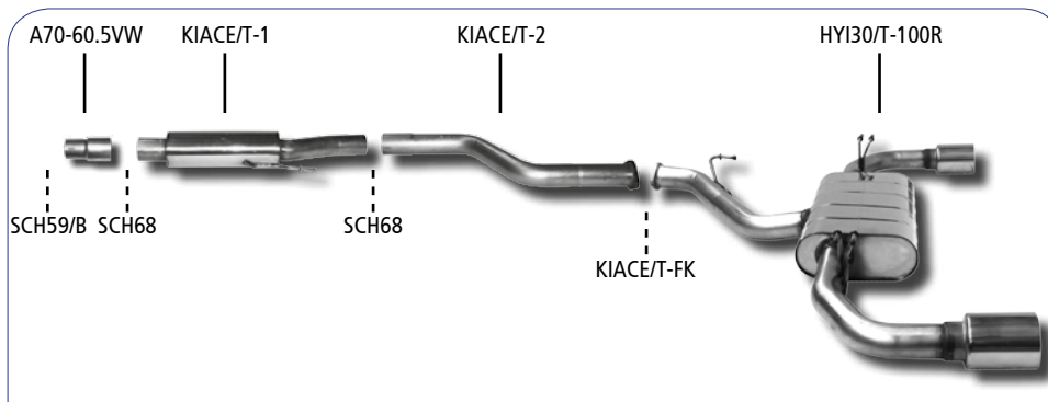
Hyundai i30 | Twin RACE | 1x Ø 100 mm gerade LH+RH |
